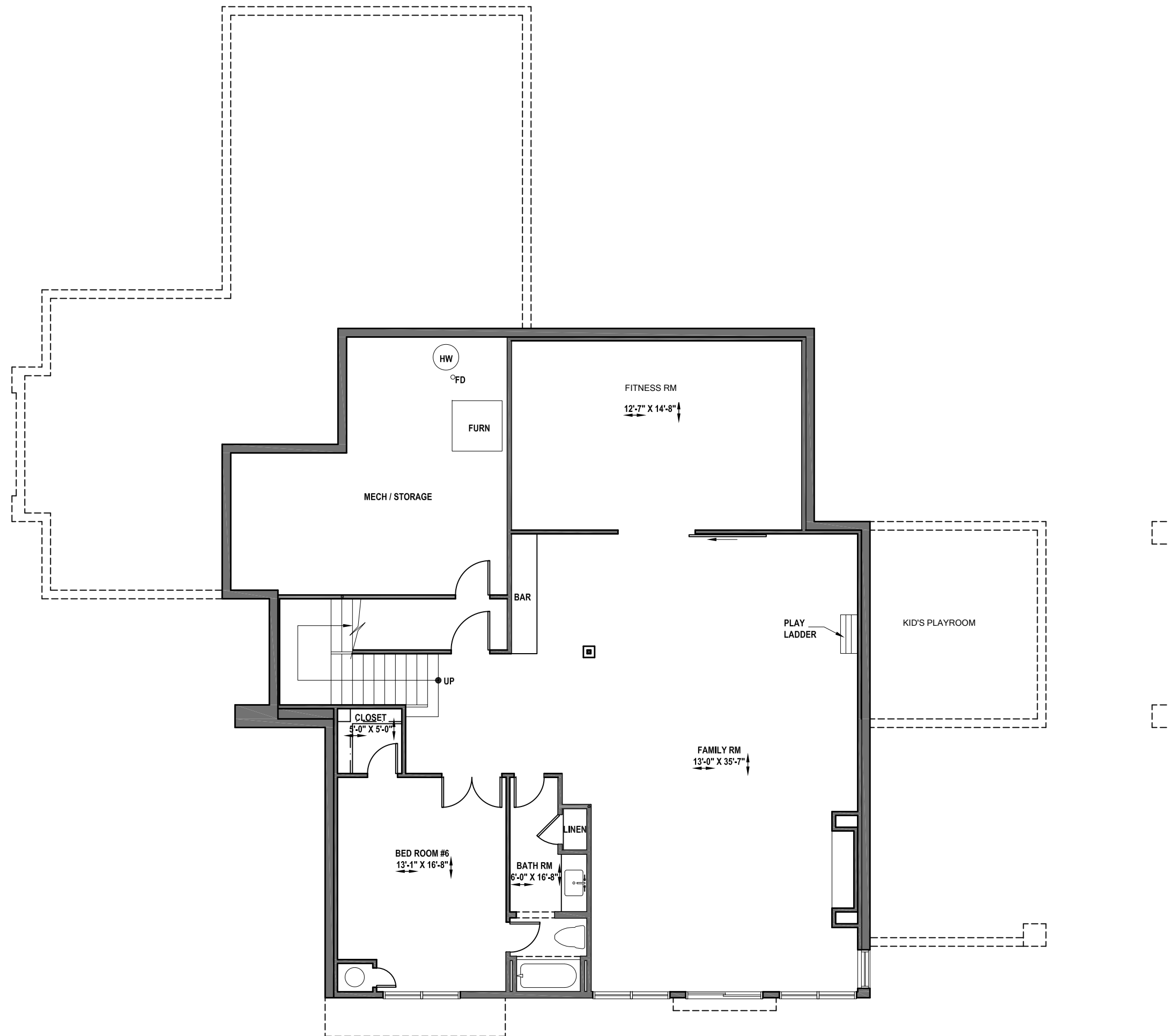
LOWER LEVEL PLAN
